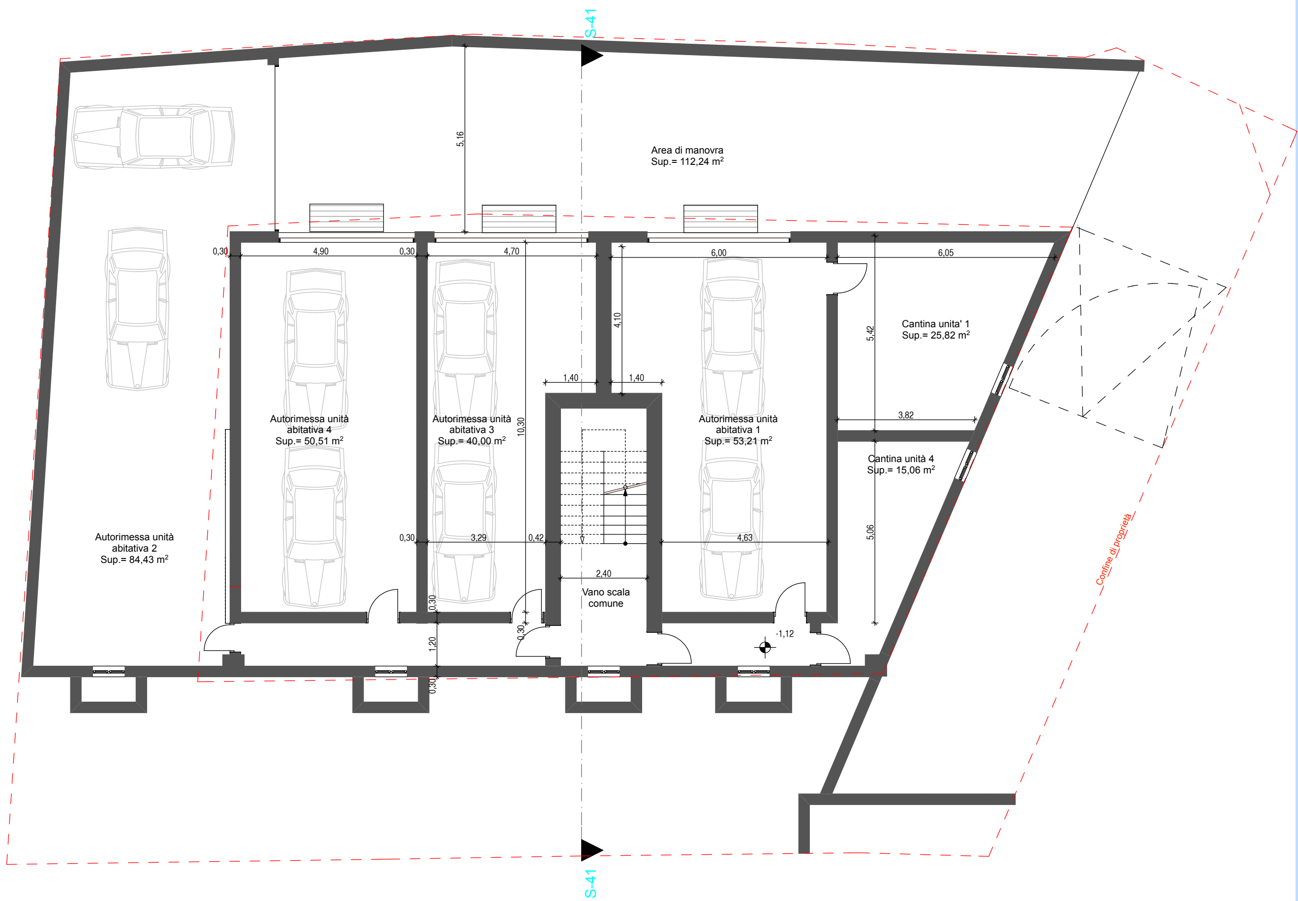
piano interrato
